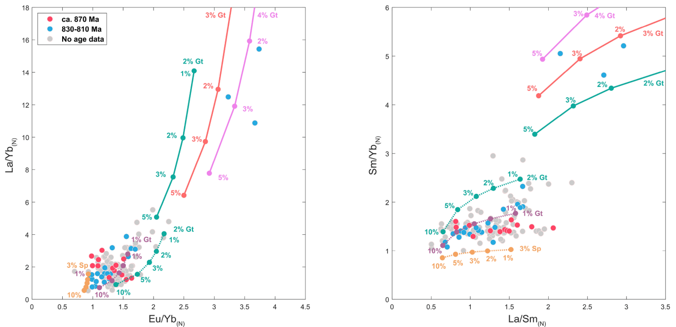
Fig. 11. Geochemical diagrams for the investigated mafic rocks. Plots of (A) \text{Eu/Yb}_{(N)} vs. \text{La/Yb}_{(N)} and (B) \text{La/Sm}_{(N)} vs. \text{Sm/Yb}_{(N)} for mafic rocks from the Dahongshan area. The melt curves are calculated based on the fractional melting model (after Lee et al., 2012) and circle marks along the curves represent the degree of partial melting. The dotted curves represent the melting of enriched DMM sources (Workman and Hart, 2005). The solid curves represent the melting of garnet-bearing lherzolite mantle sources (Jourdan et al., 2007). The Chondrite-normalized data are after Sun and McDonough (1989). Partition coefficients and modal proportions for spinel peridotite, garnet peridotite and garnet-bearing lherzolite are taken from Mckenzie and O’Nions (1991) and Jourdan et al. (2007). Data sources are the same as those in Fig. 5.
