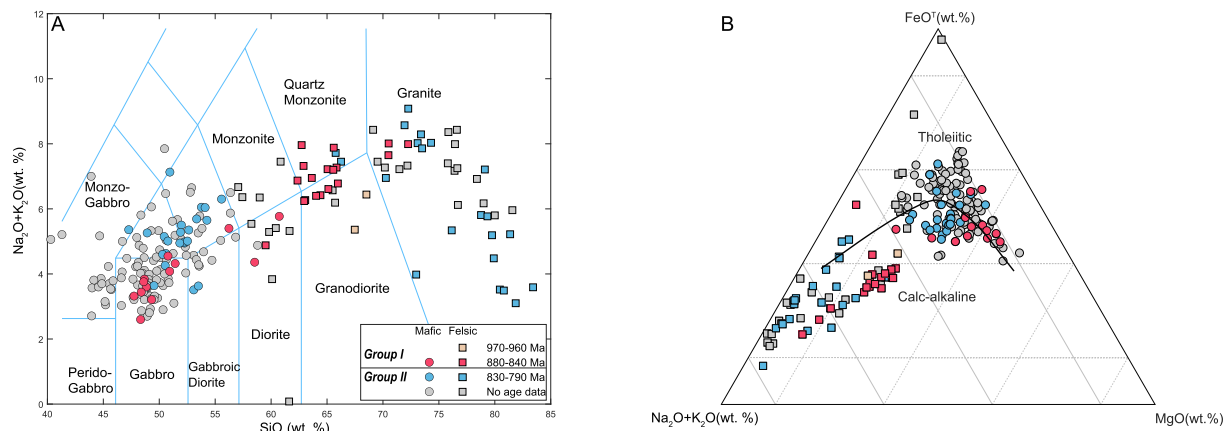
Fig. 5. Rock classification diagrams for the igneous rocks from the Dahongshan area. (A) Total alkali vs. silica diagram. (B) (\text{Na}_2\text{O} + \text{K}_2\text{O})\text{-FeO}^*\text{-MgO} (AFM) plot from Irvine and Baragar (1971). Data sources are from Dong et al. (1999), Dong (2004), Shi et al. (2003, 2005), Deng et al. (2013), Hu et al. (2015a, 2017), Liao et al. (2016), Xu et al. (2016), Chen et al. (2017), Yang (2017), Xie et al. (2019), Liu and Zhao (2019), Liu et al. (2020, 2022) and this study.
